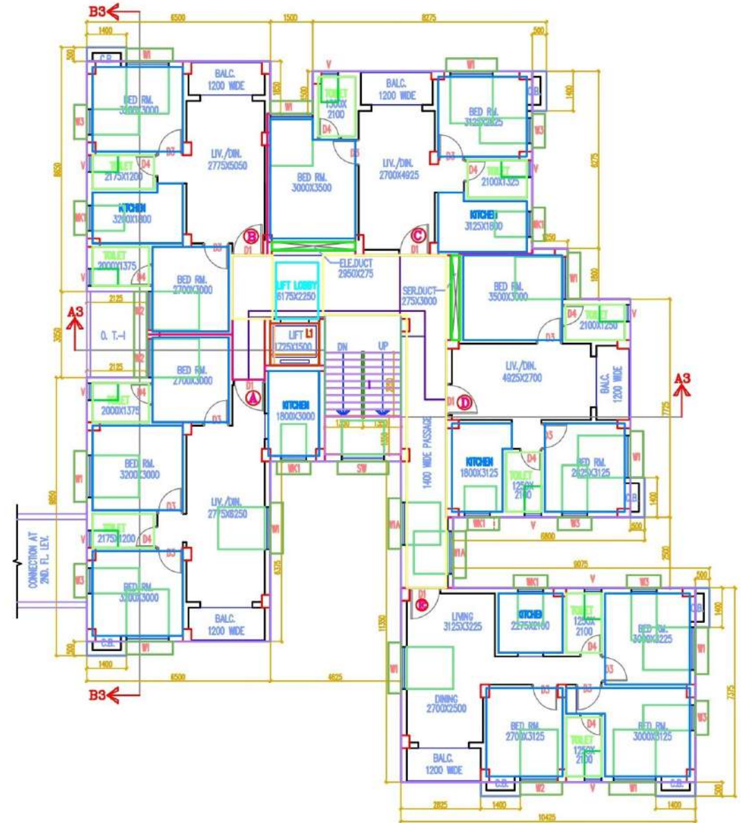
FLOOR01,FLOOR02,FLOOR03,FLOOR04-TYPICAL
